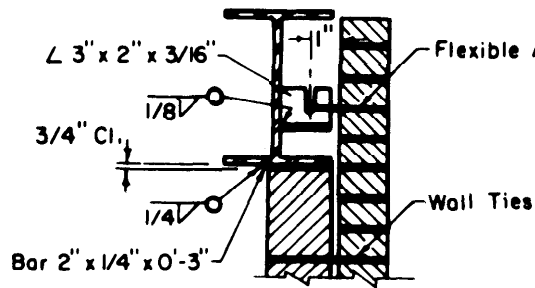
WALL ANCHORAGE TO STEEL BEAM *
