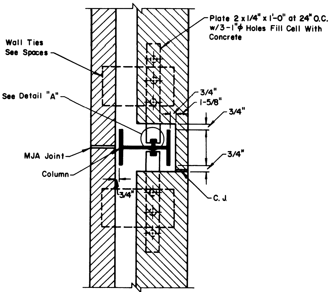
Figure C-3. (Sheet 2 of 2).
